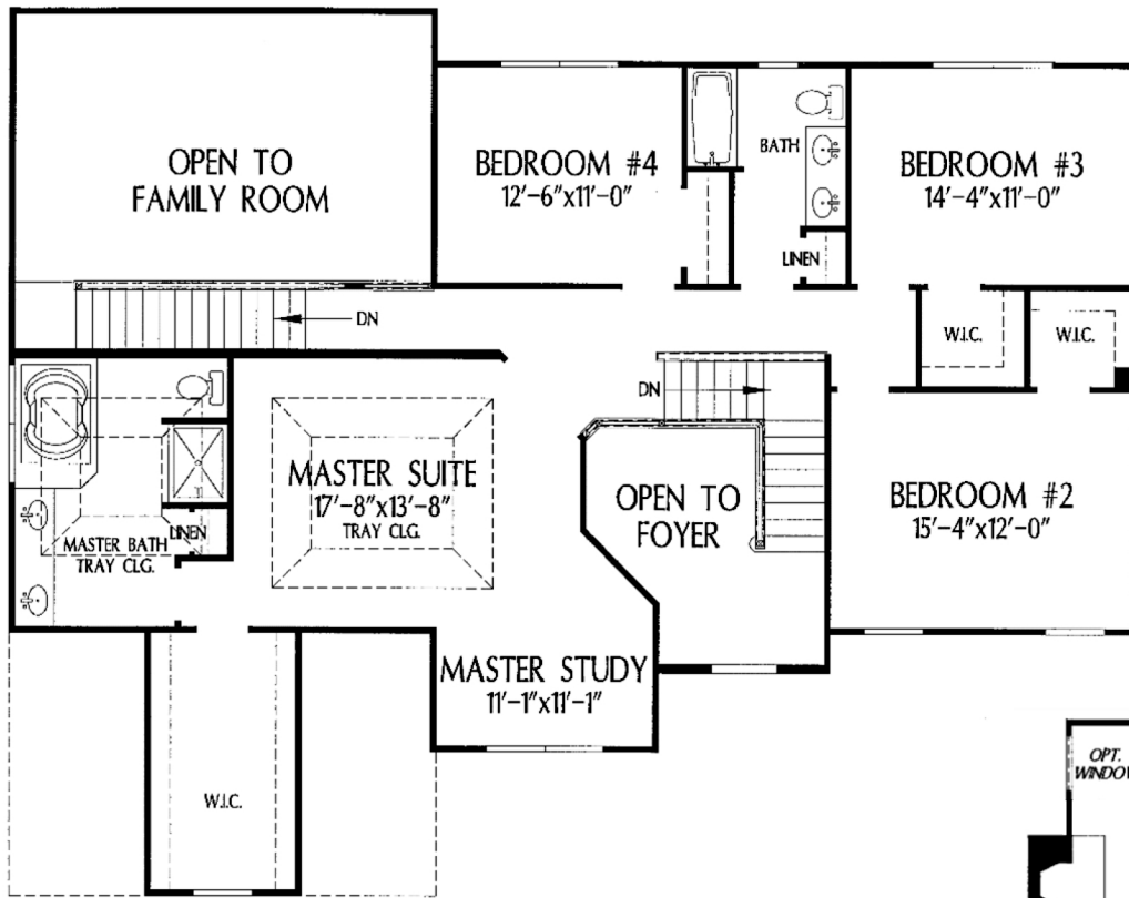
Second Floor
